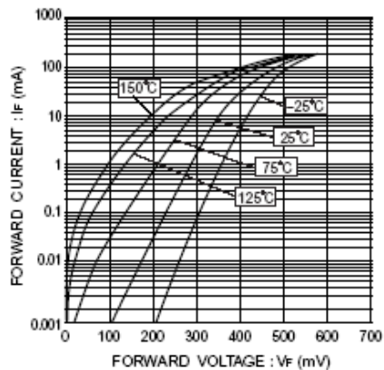
Fig.1 Forward characteristics
